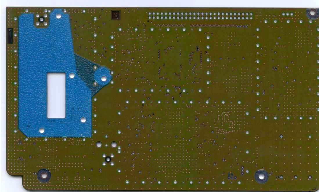
BRU3902 FRB (radio board) blank PCB, bottom side
