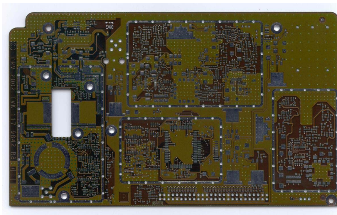
BRU3902 FRB (radio board) blank PCB, top side
