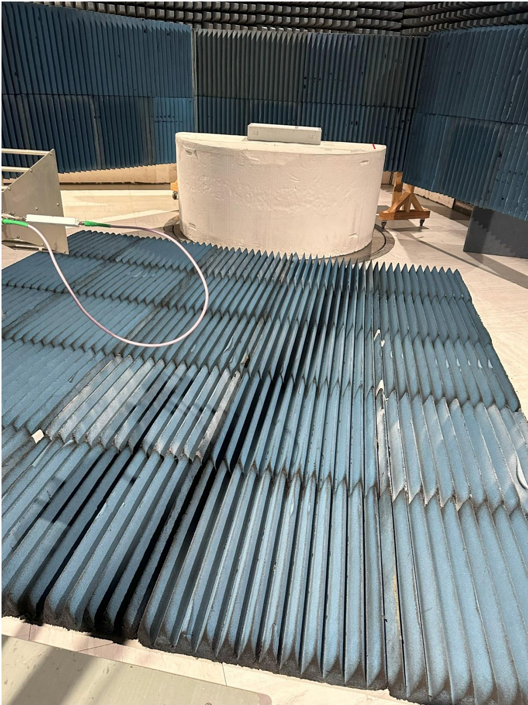
Radiated emissions
