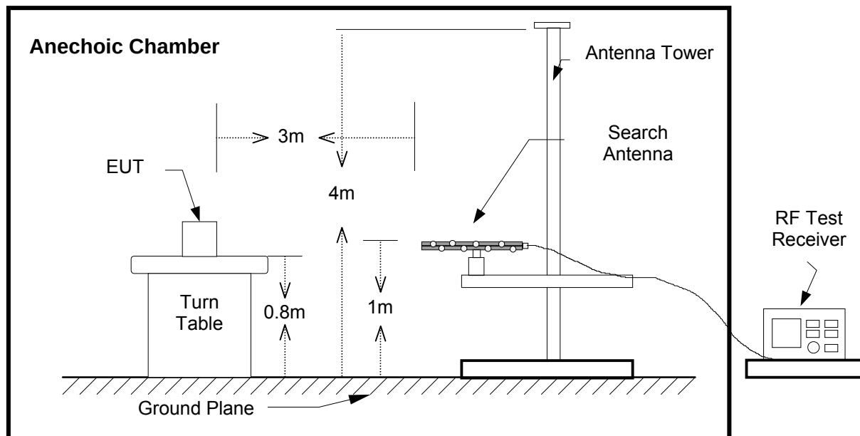
Test Set-Up 3 Figure 1: Frequencies measured below 1 GHz configuration
