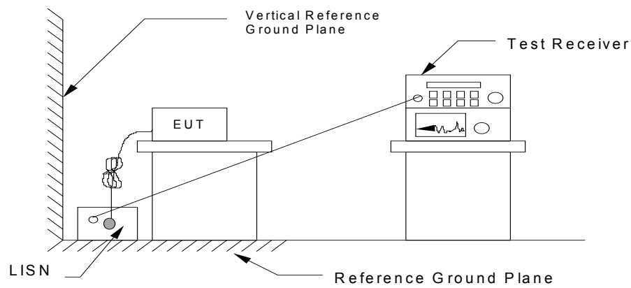
Test Set-Up 4
