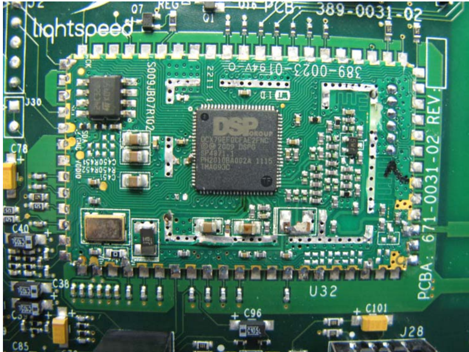
Speaker Oscillator PCB comp side (View 2)
