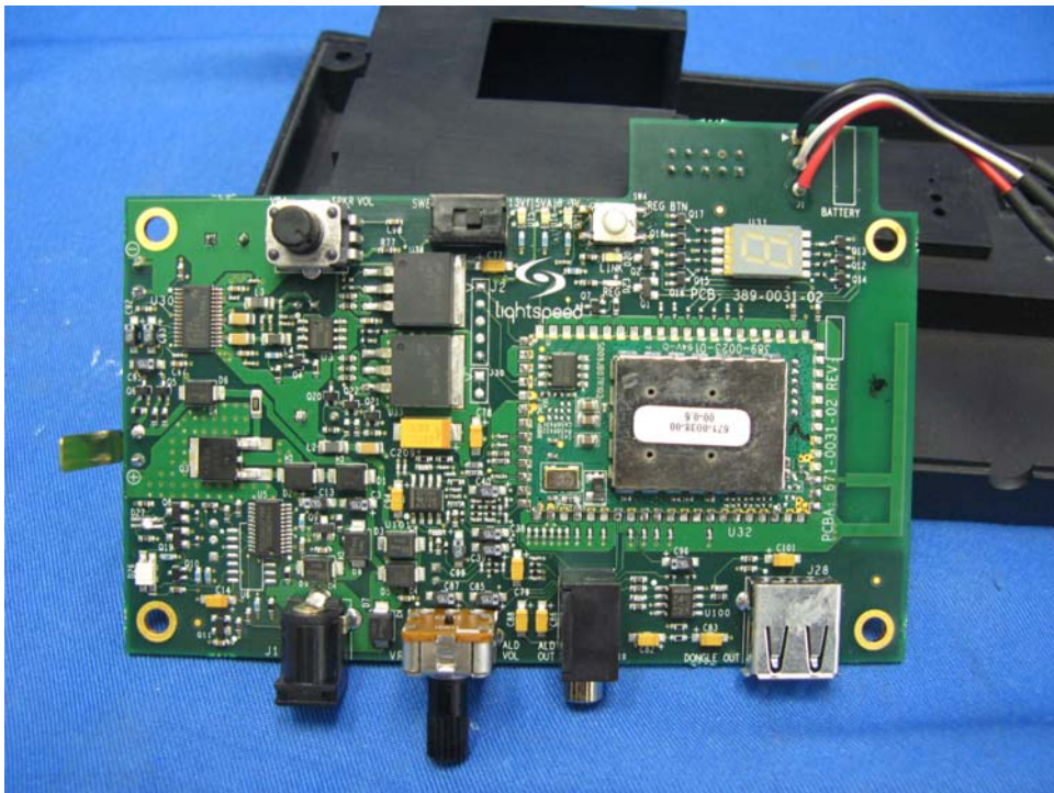
Speaker Main PCB comp side (View 1)
