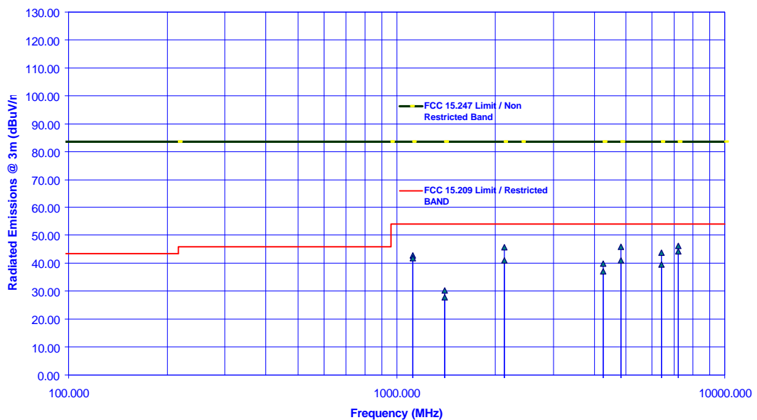
Transmitter Radiated Emissions Measurements at 3 Meter OFTS NgeeAnn Polytechnic, INLink Wireless LAN Card, Model INLink-2000 TRANSMIT Freq.: 2412 MHz
