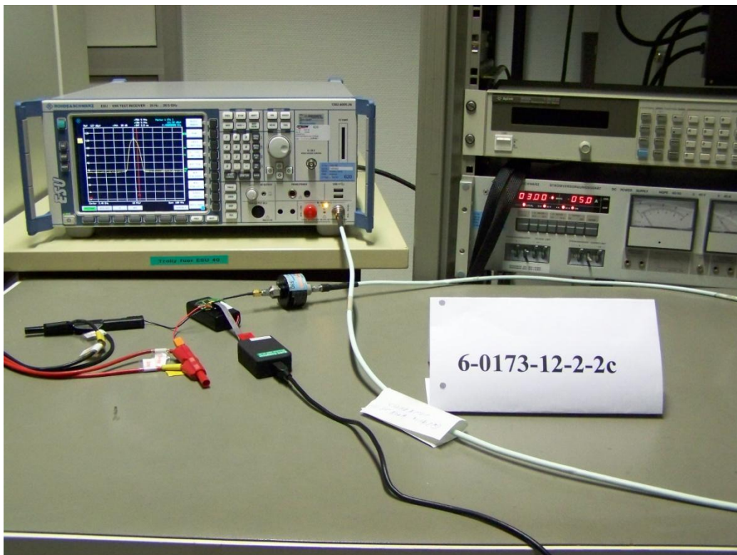
Conducted RF-measurements at the Radio laboratory 1 (in the climatic chamber), test setup 2
