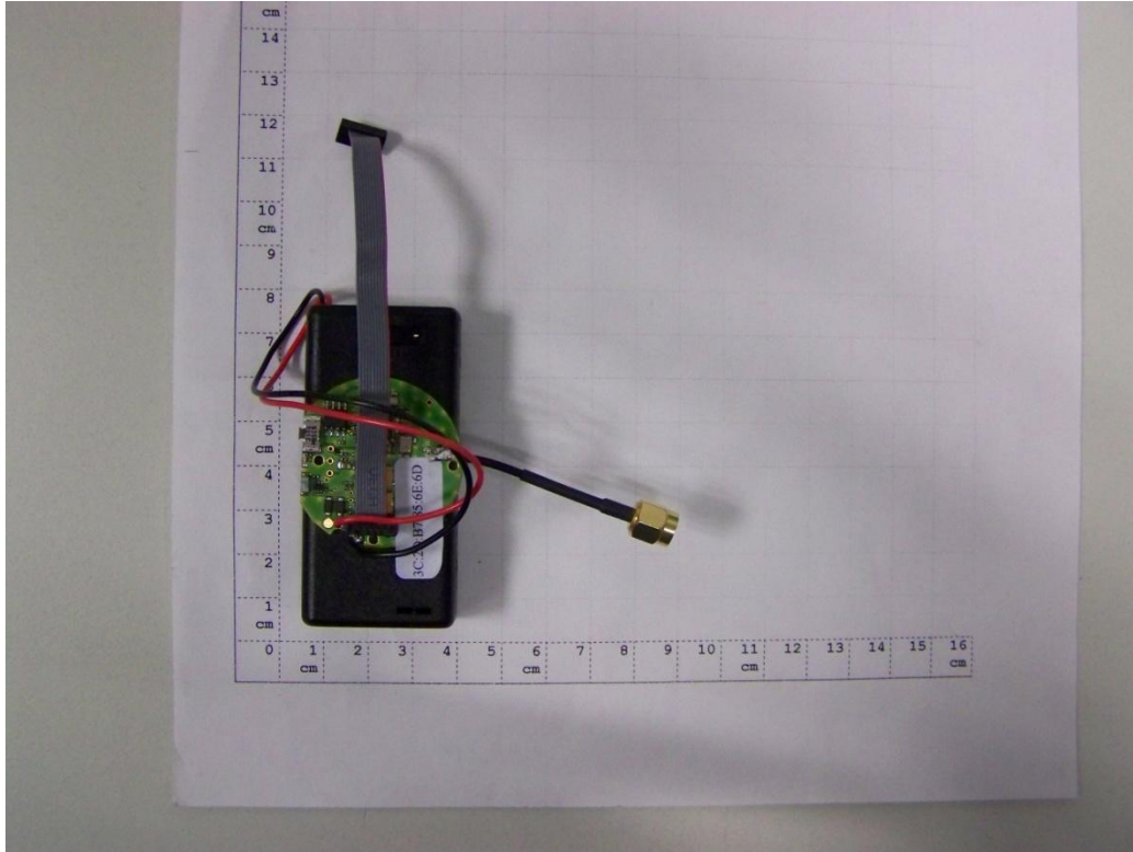
EUT B top view (modified for conducted tests)
