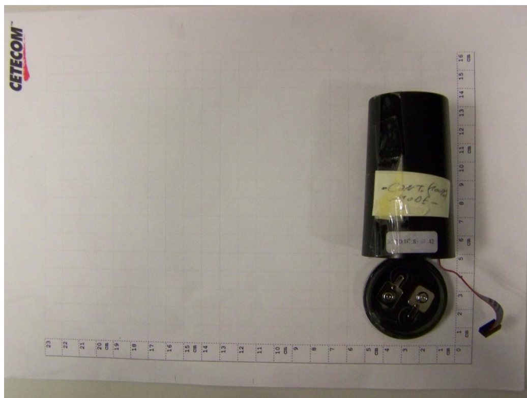
EUT A with bottom end cap
