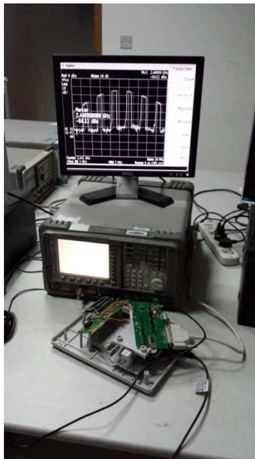
SPURIOUS EMISSION TEST SETUP
