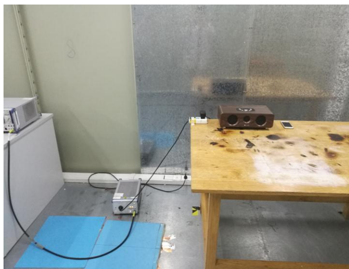
Conducted Emission
