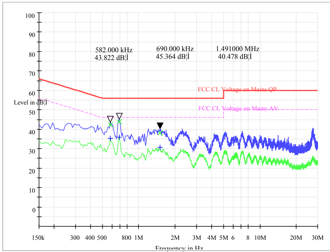
FCC CL Voltage Test
