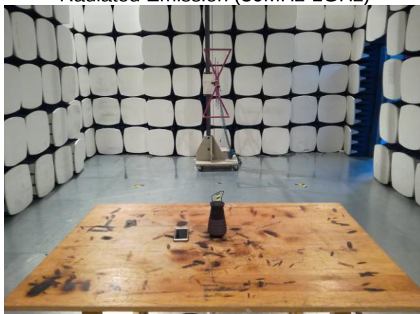
Radiated Emission (30MHz-1GHz)
