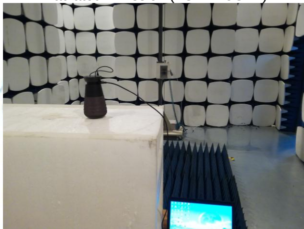
Radiated Emission (1GHz-25GHz)
