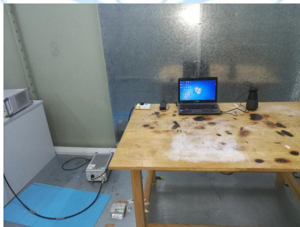
Conducted Emission
