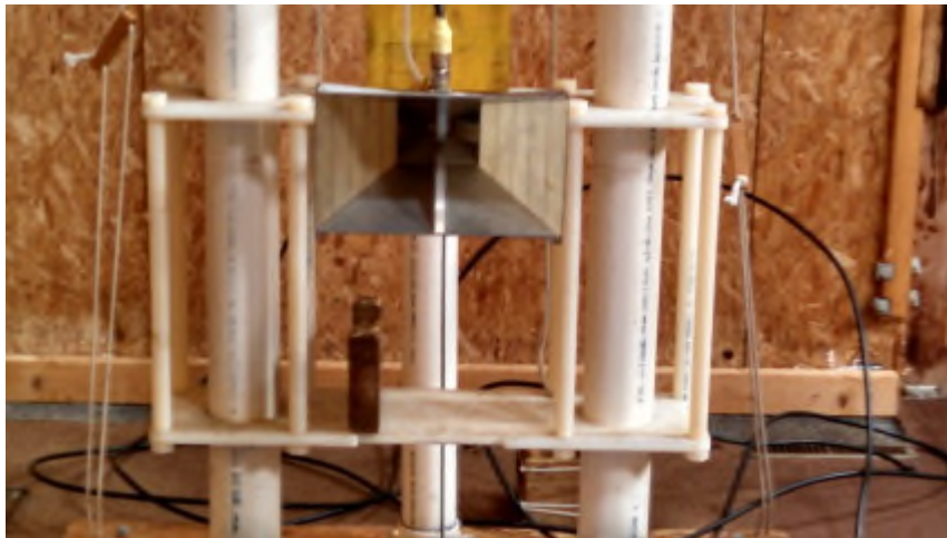
3115 Ridged Horn Antenna
