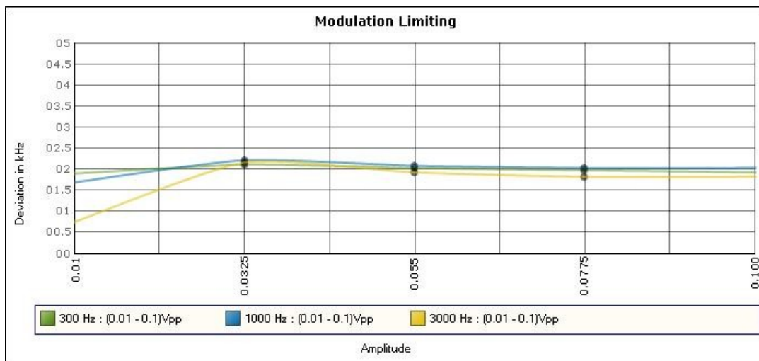
Modulation Limiting Plot – Wide band
