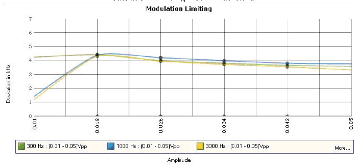
Modulation Limiting Plot – Wide band
