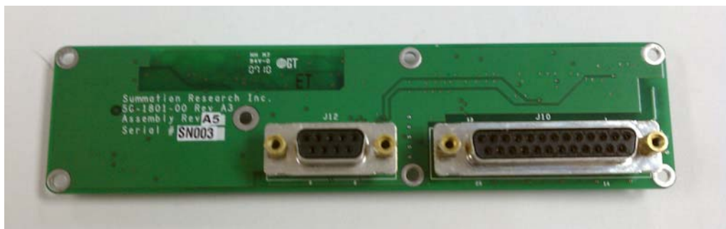
Figure 5 Front Panel Card (FPC), Rear
