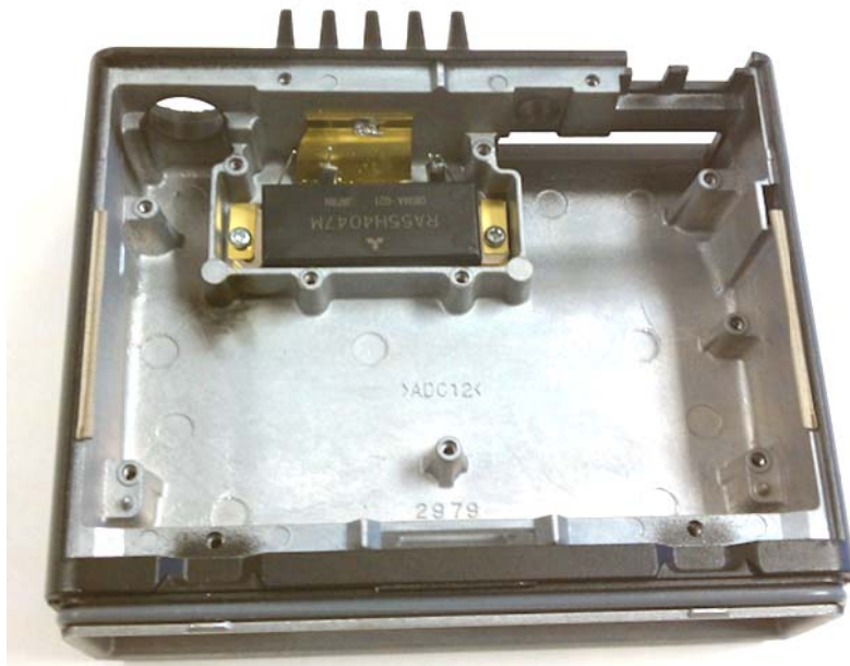
Figure 8 Radio Chassis with Power Amplifier
