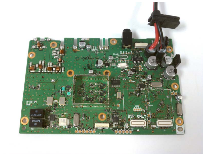
Figure 3 Main Board, Top, No Shields
