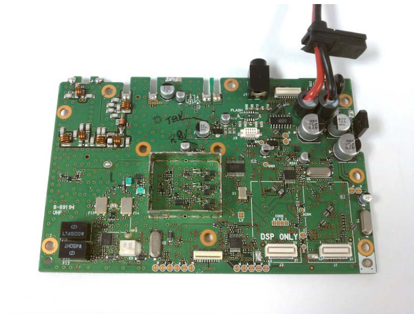
Figure 7 Modem Data Card (MDC), Rear
