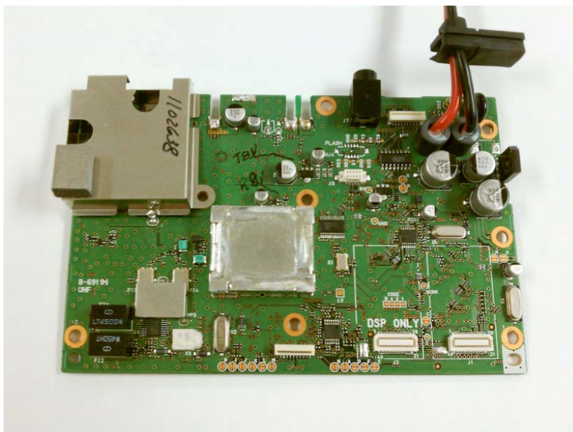
Figure 2 Main Board, Top, with Shields
