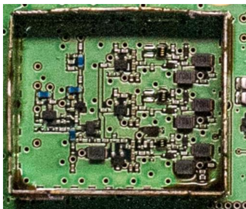
Transmit Receive Main Card Top, Detail Under Shield
