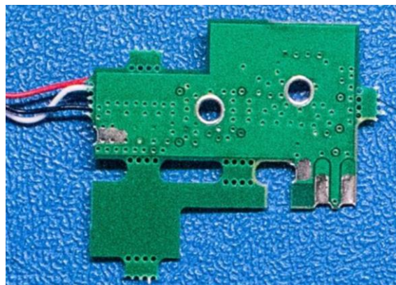
Receive signal splitter card Bottom
