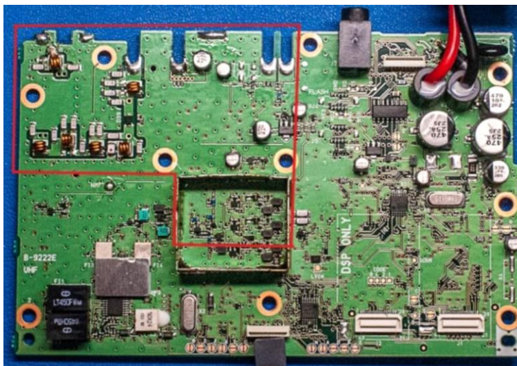
Transmit Section of Radio
