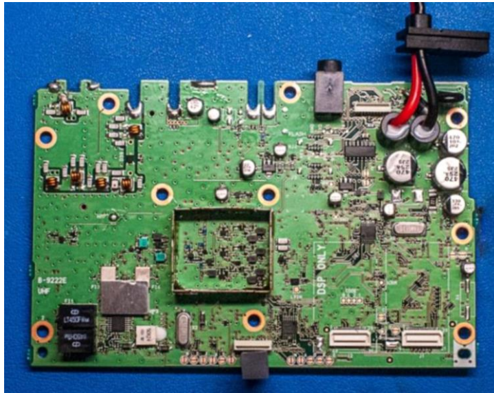
Transmit Receive Main Card Top
