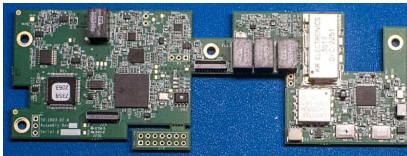
Modem Processing Card Top
