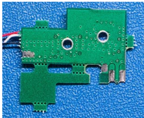
Receive signal splitter card Bottom
