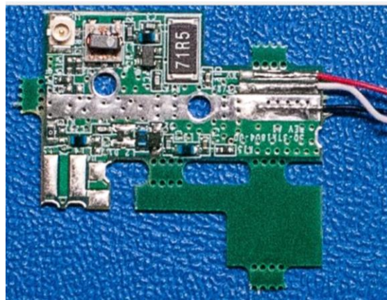
Receive signal splitter card Top
