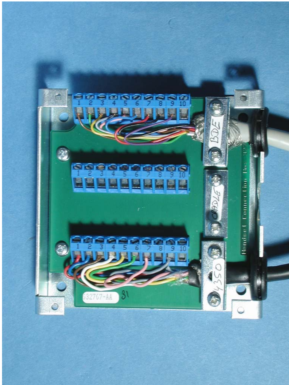
Internal of junction box
