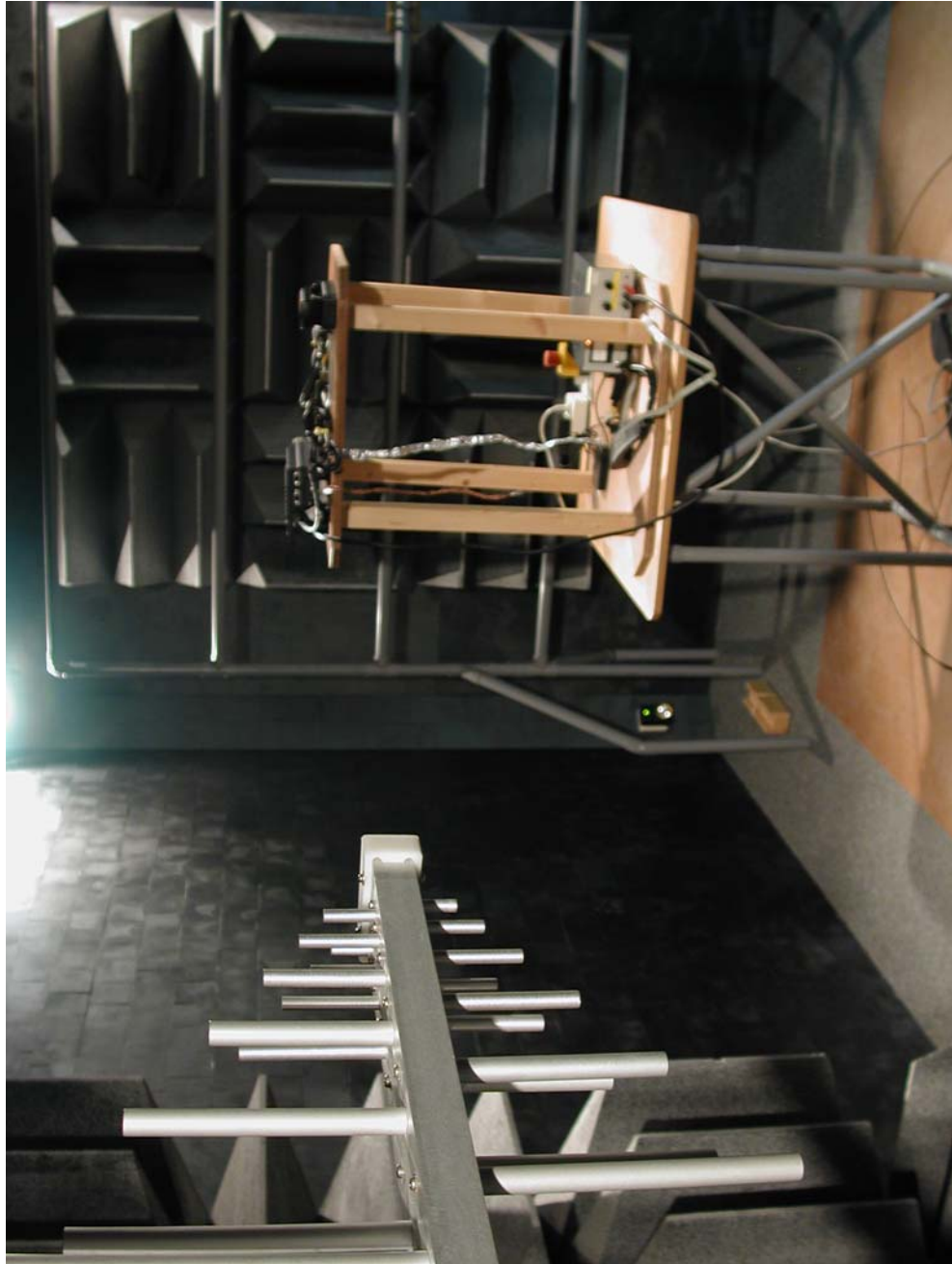
Radiated emission
