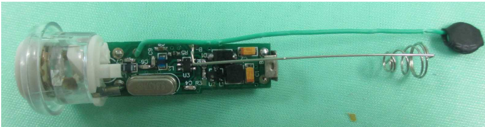
PHOTOGRAPH OF THE PRODUCT INNER CIRCUIT TOP VIEW
