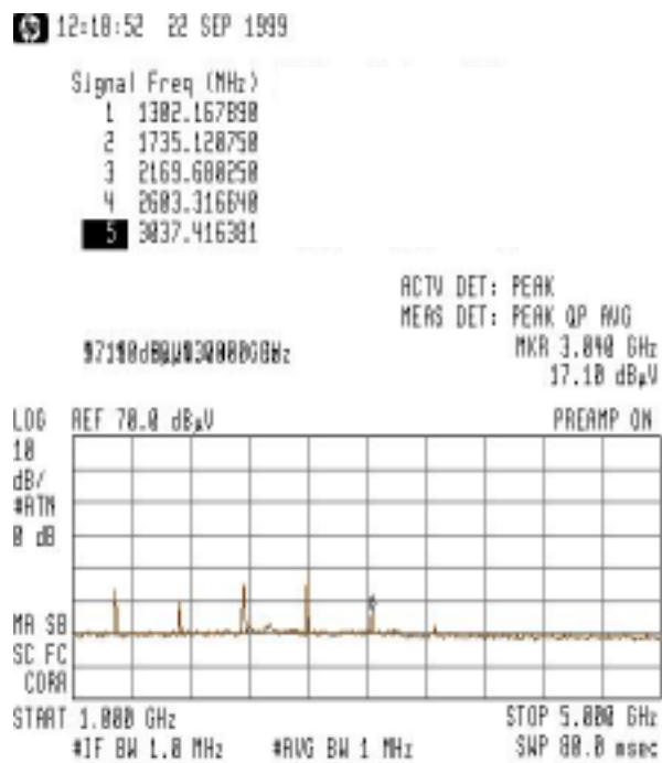
Plot of frequencies from 1 to 5 GHZ
