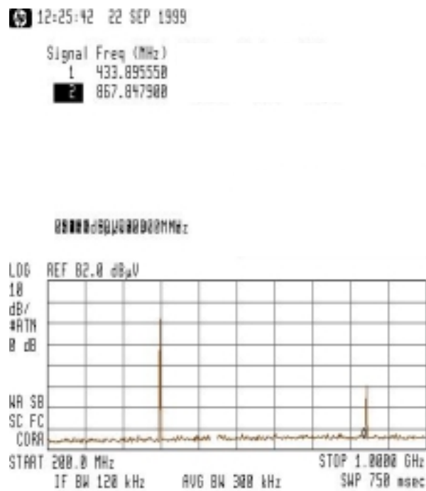
Plot of frequencies from 200 to 1000 MHZ
