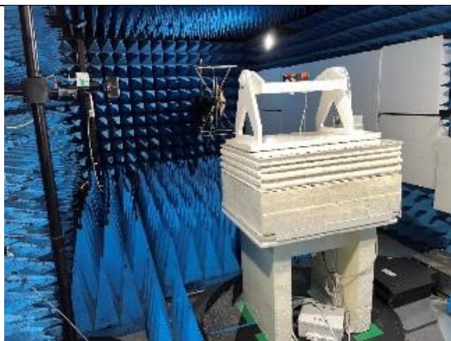
Test Setup above 1GHz
