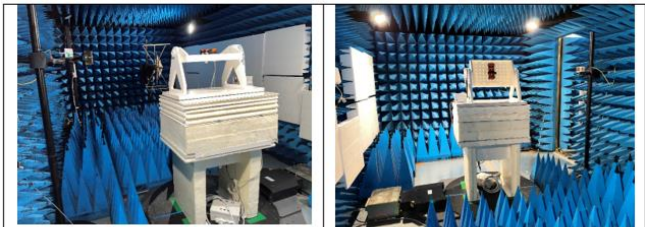
Test Setup above 1GHz
