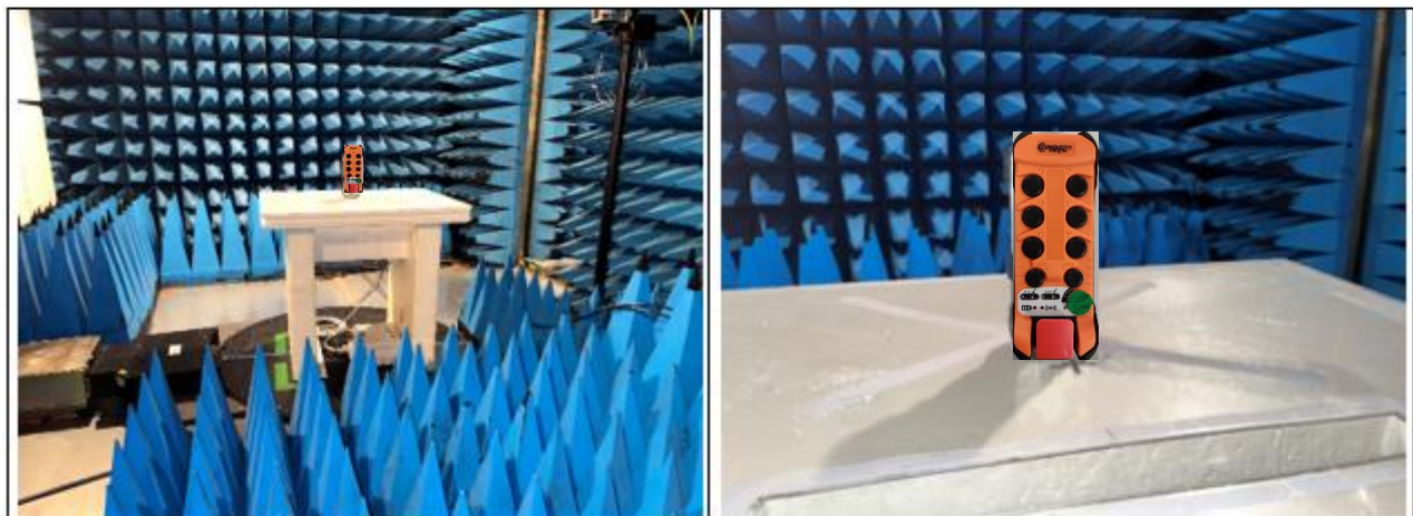
Test setup under 1GHz
