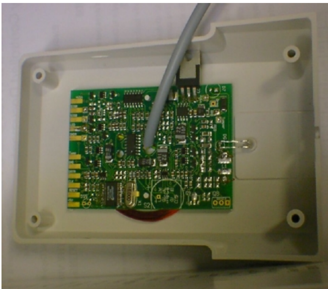
PCB Assembly (Component Side)
