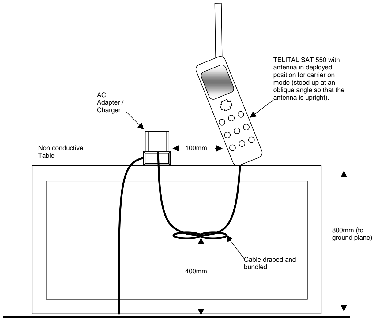
Figure 4: Telital SAT 550 CFR 47 Part 25.202(f) Radiated Emission Set up (Rear View)
