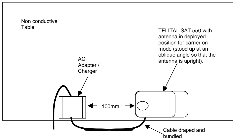
Figure 5: Telital SAT 550 CFR 47 Part 25.202(f) Radiated Emission Set up (Plan View)
