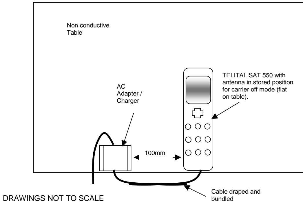
Figure 3: Telital SAT 550 CFR 47 Part 15.109 Radiated Emission Set up (Plan View)
