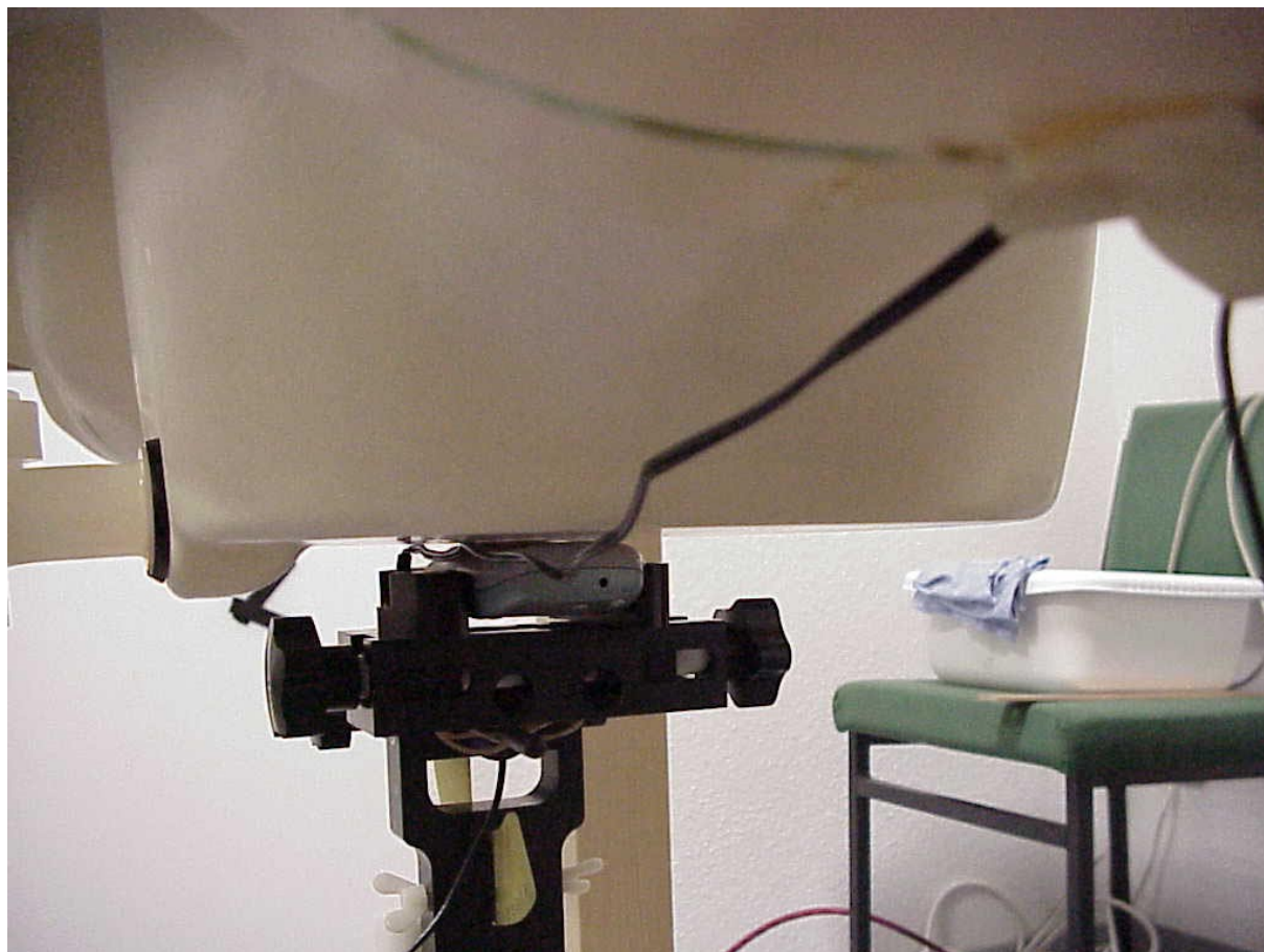
Photo 4: Body measurement (flat phantom)
