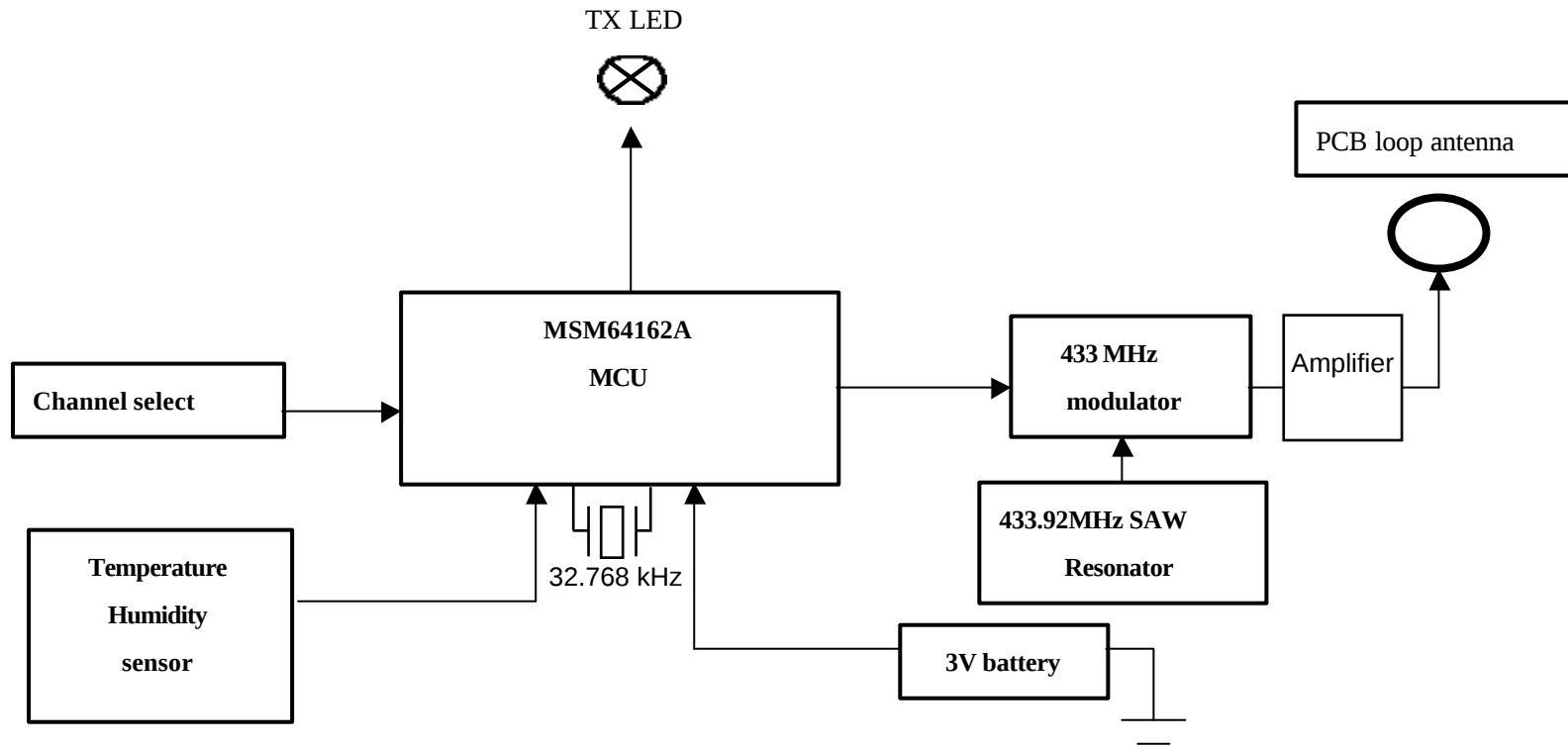
Figure 1 C8102 Block diagram
