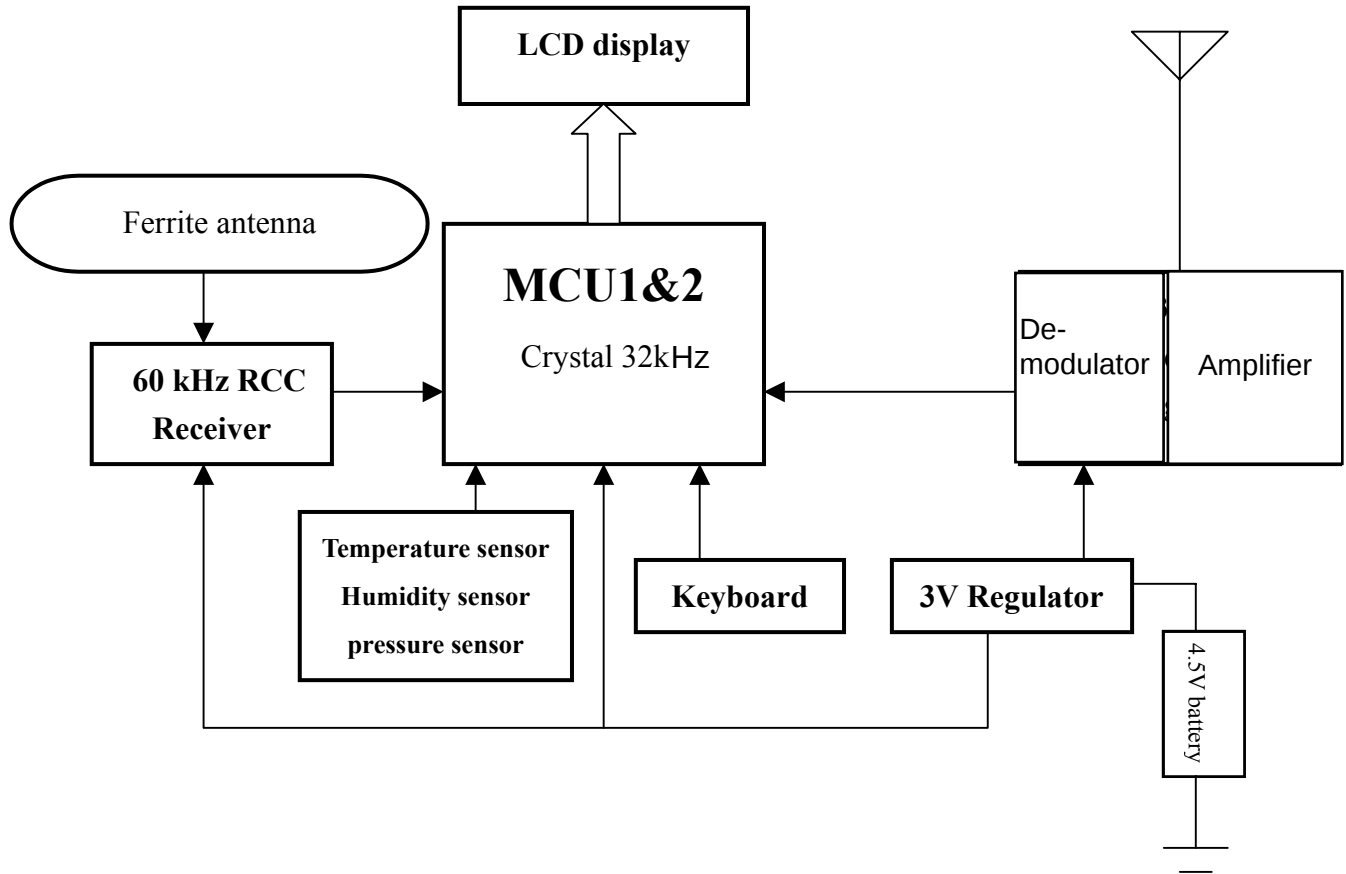
Figure 1 C-8136 Block diagram
