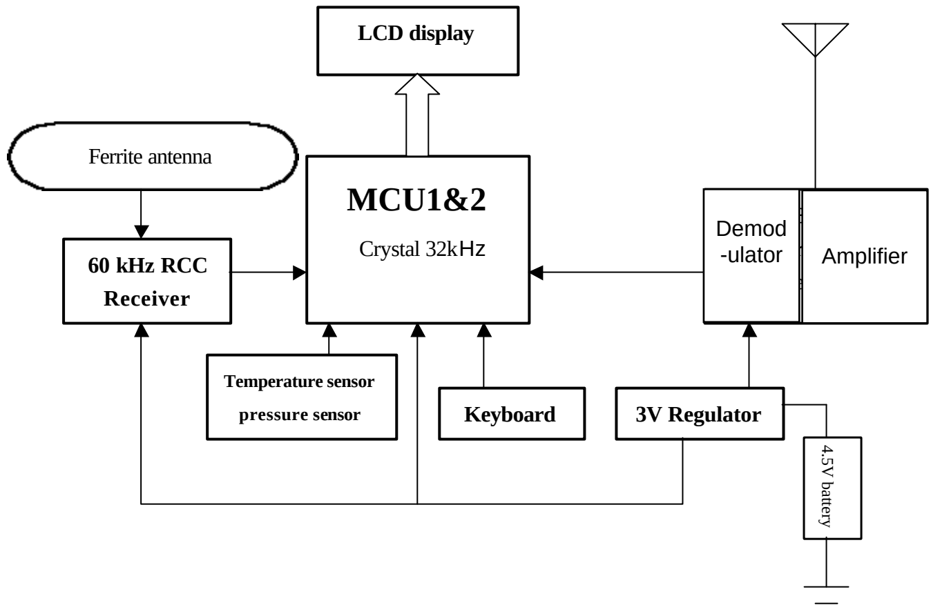
Figure 1 C-8154 Block diagram
