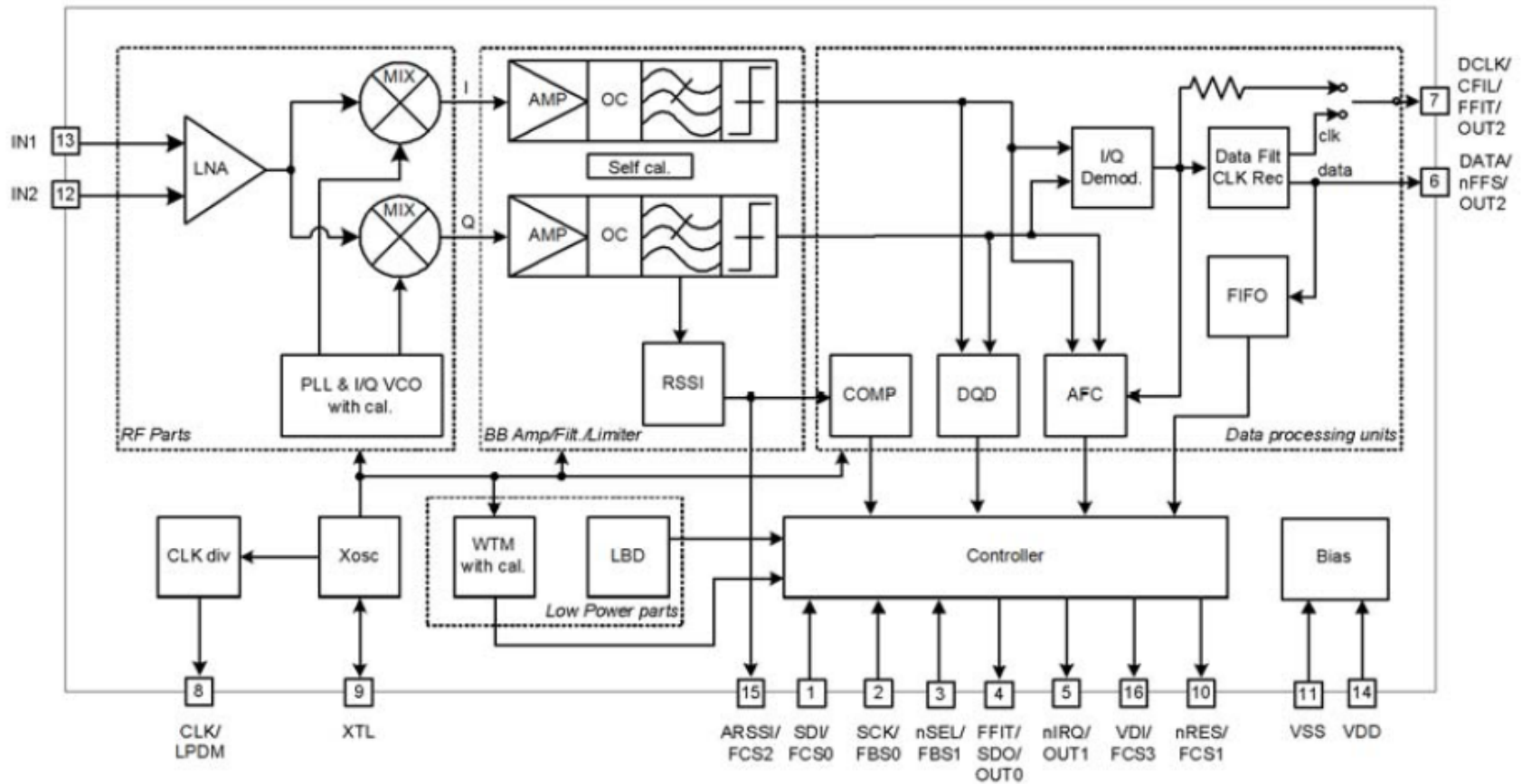
RF Receiver RF227 Block Diagram
