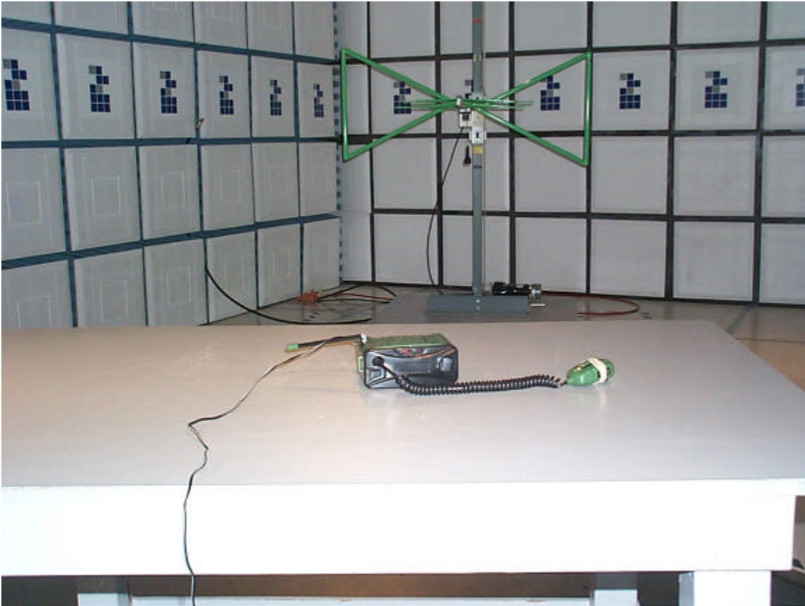
Maximized Radiated Emission Test Set-up Front View - Horizontal
