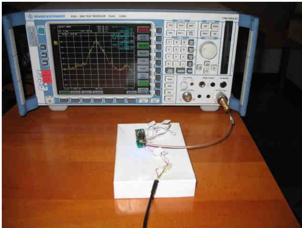
Photograph 3: Set-up for Transmitter test
