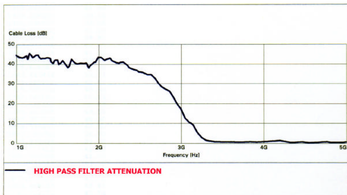
(o) Trilithic High Pass Filter
