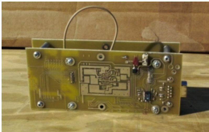
(b) Module – Bottom View
