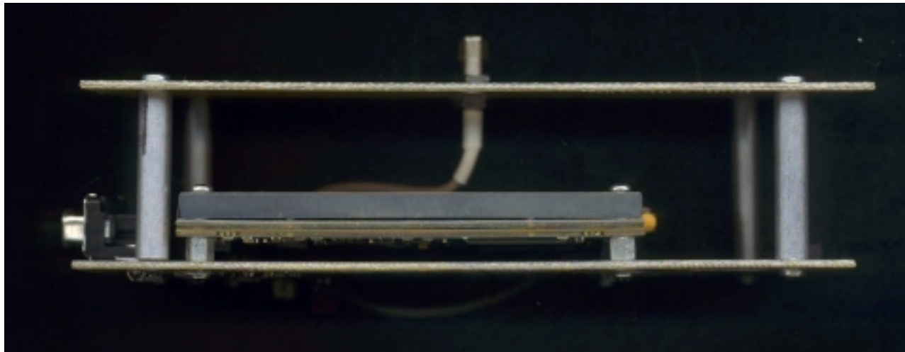
(f) Module – Side View I
