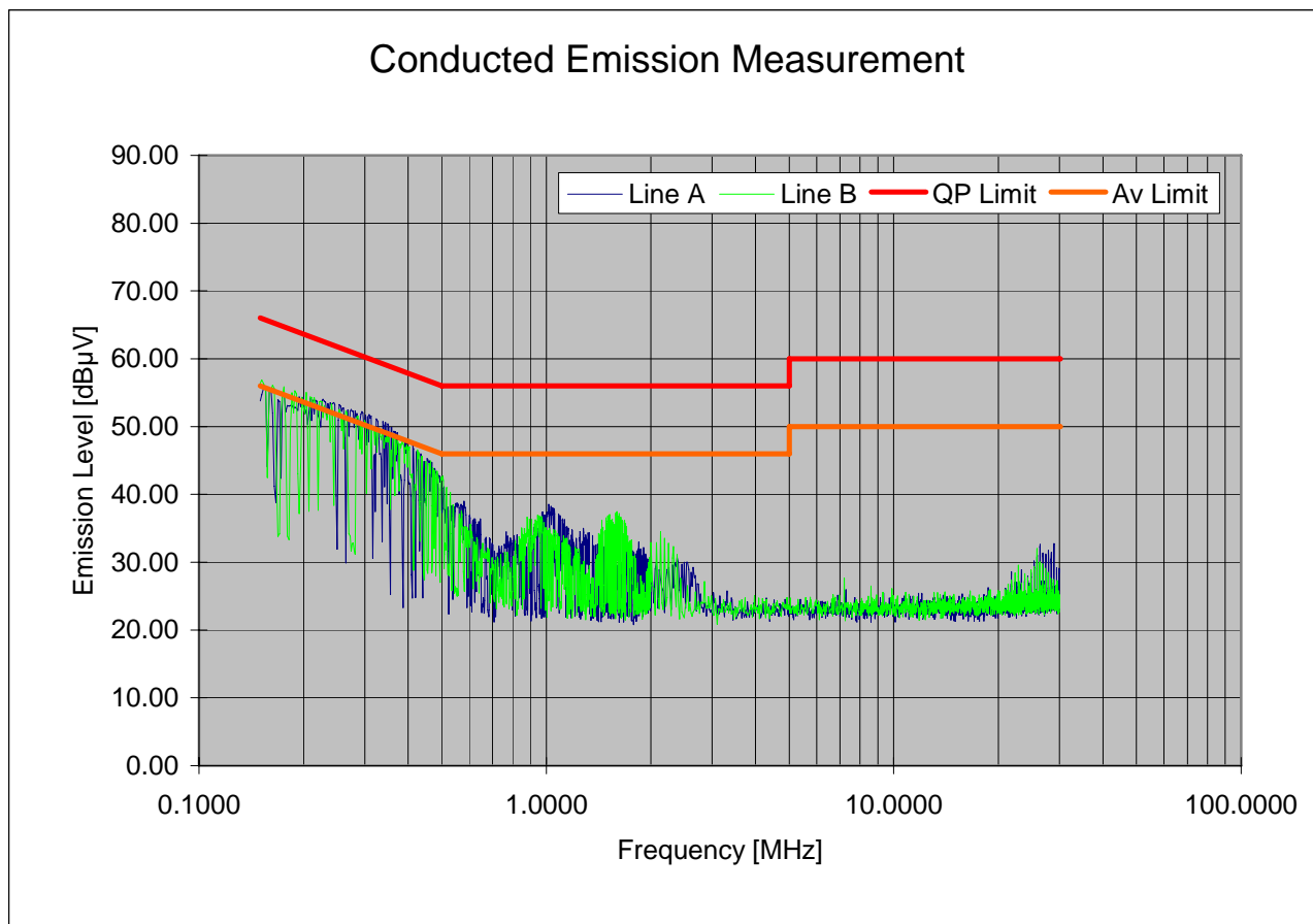
Plot 6-39. Line Conducted Plot with 802.11a
