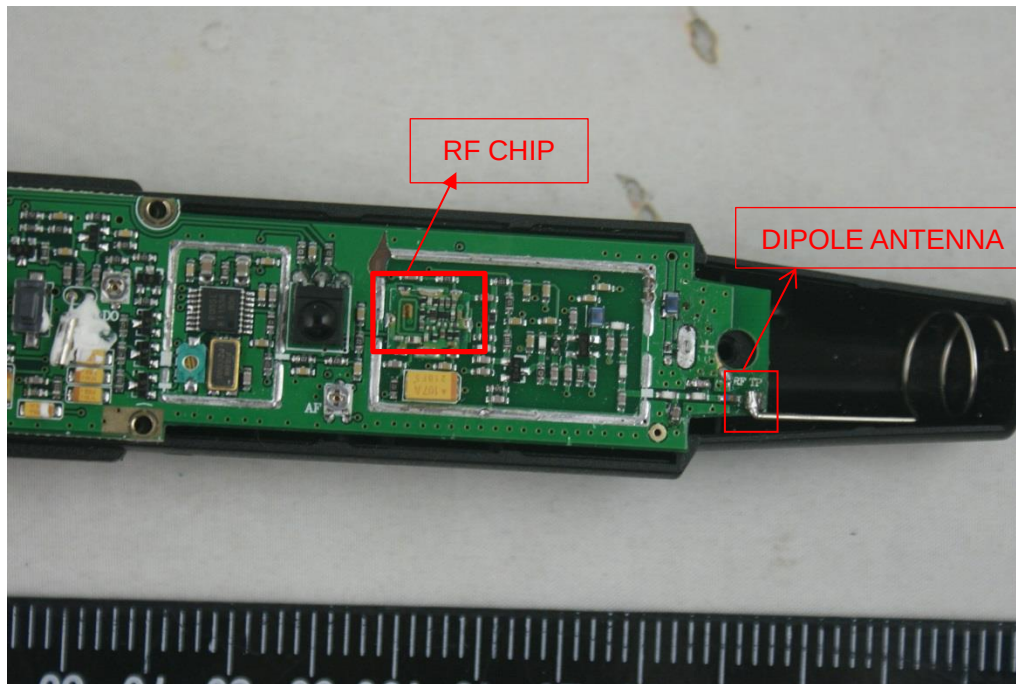
MAIN BOARD 1 FRONT DETAIL VIEW
