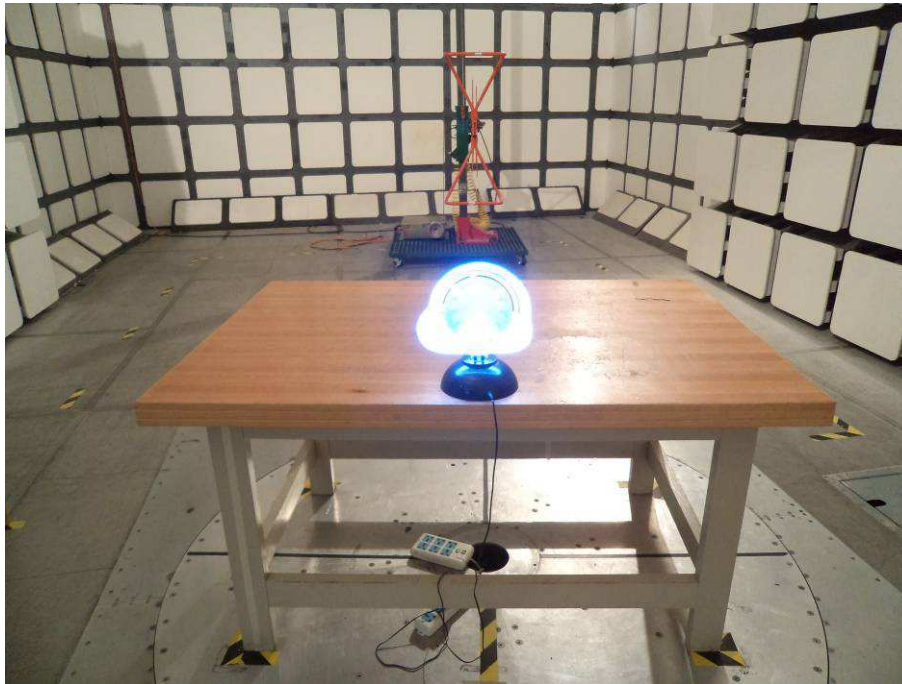
Radiated Emissions View (Model: NL-1203)
