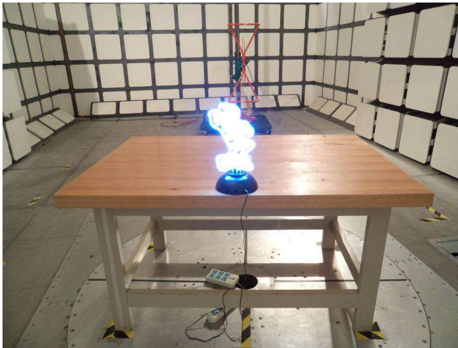
Radiated Emissions View (Model: NL-1206)
