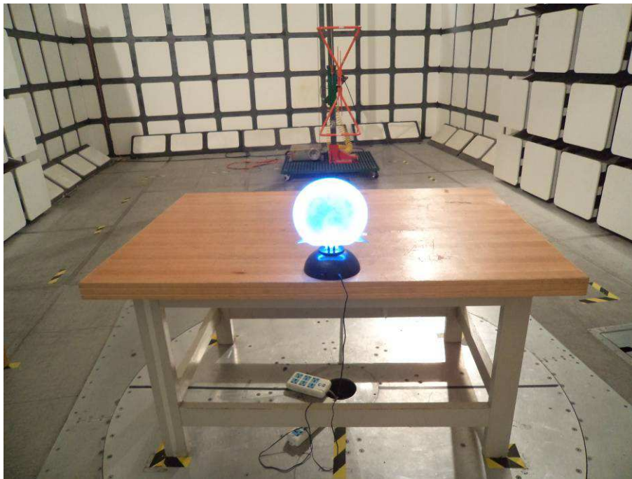
Radiated Emissions View (Model: NL-1204)
