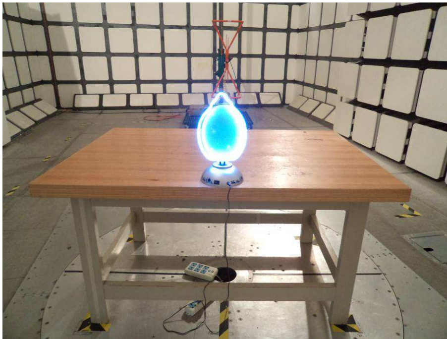
Radiated Emissions View (Model: NL-1208)
