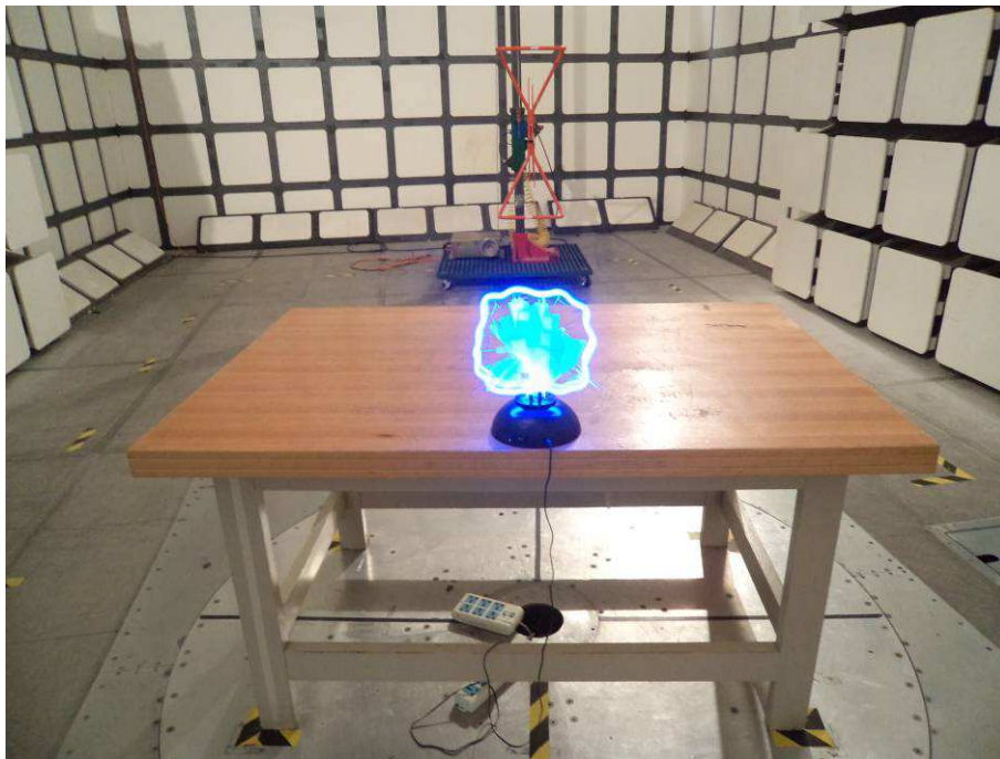
Radiated Emissions View (Model: NL-1202)
