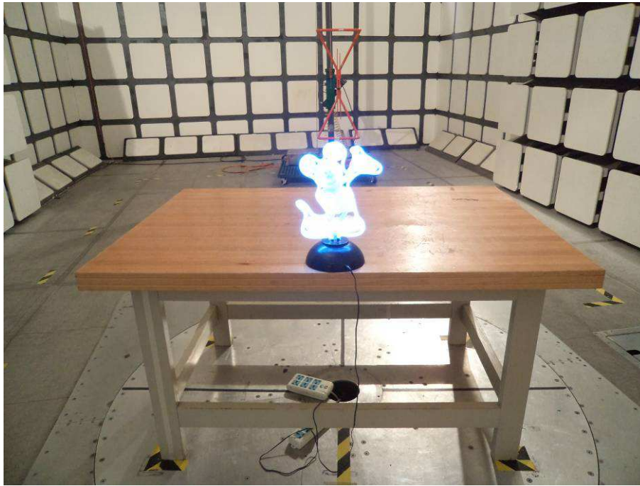
Radiated Emissions View (Model: NL-1205)
