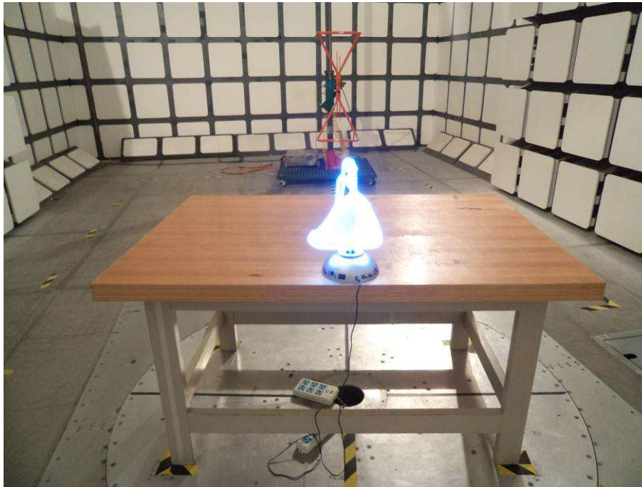
Radiated Emissions View (Model: NL-1207)
