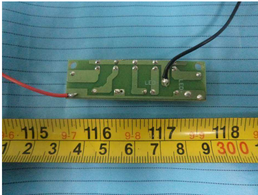
EUT – RK12-18-4 Board Bottom View
