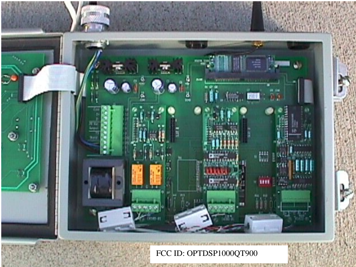
Internal View of Transmitter
