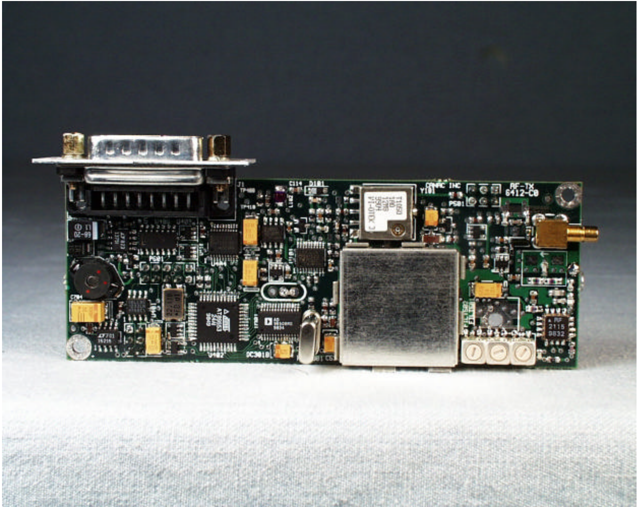
Component side of the board (with RF cans installed)
