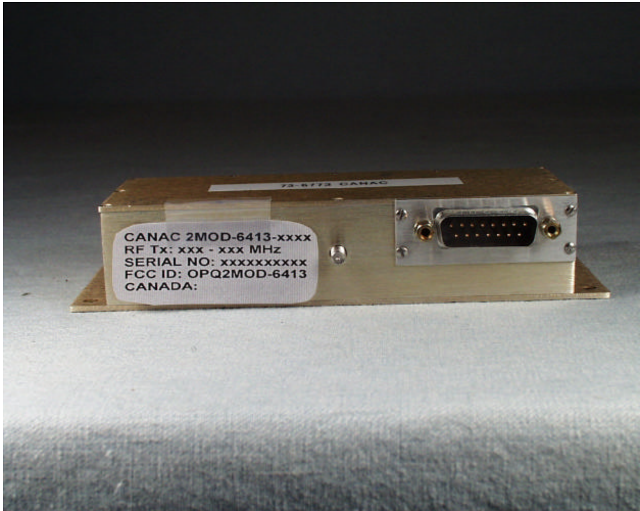
End View of the 2MOD-6413-xxxx showing the RS-232 connector
