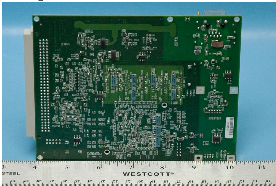
CtrlBoard_Back
