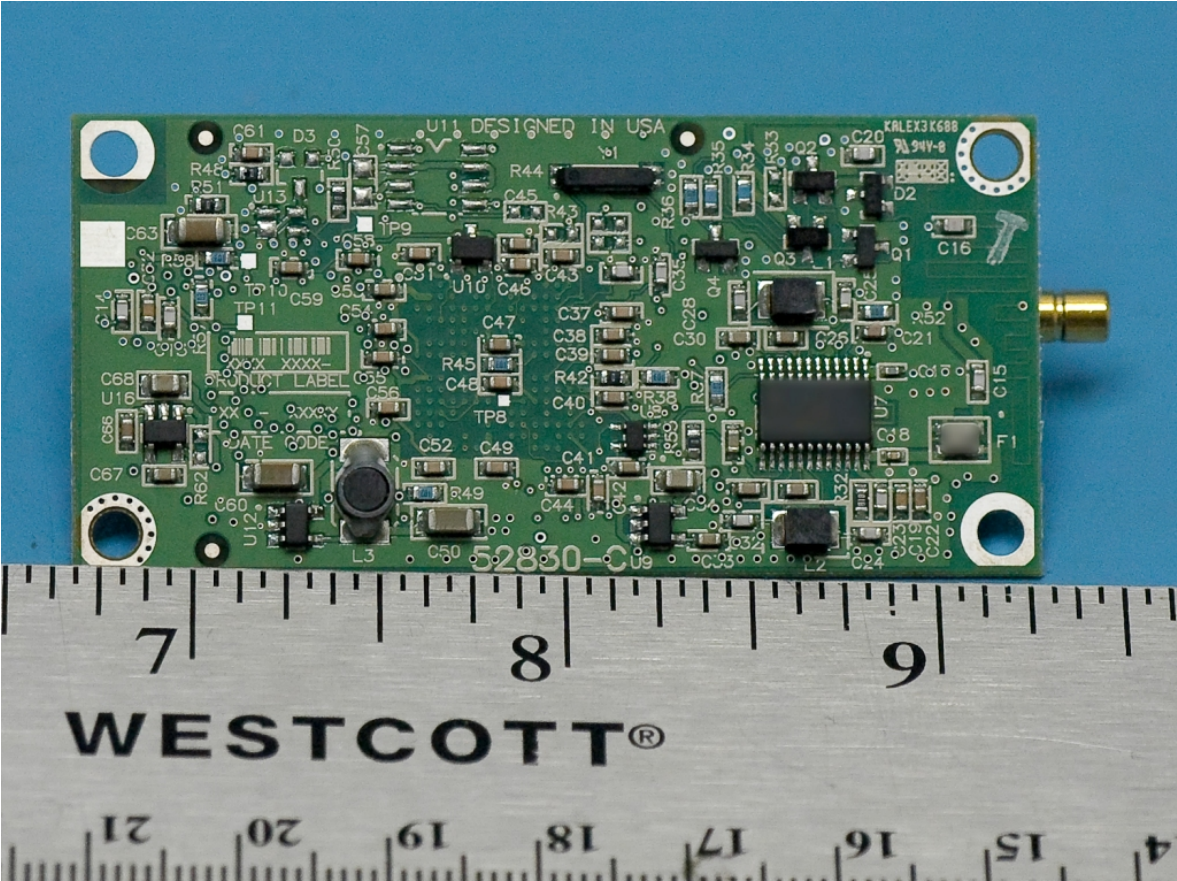
SubBoard-Back
