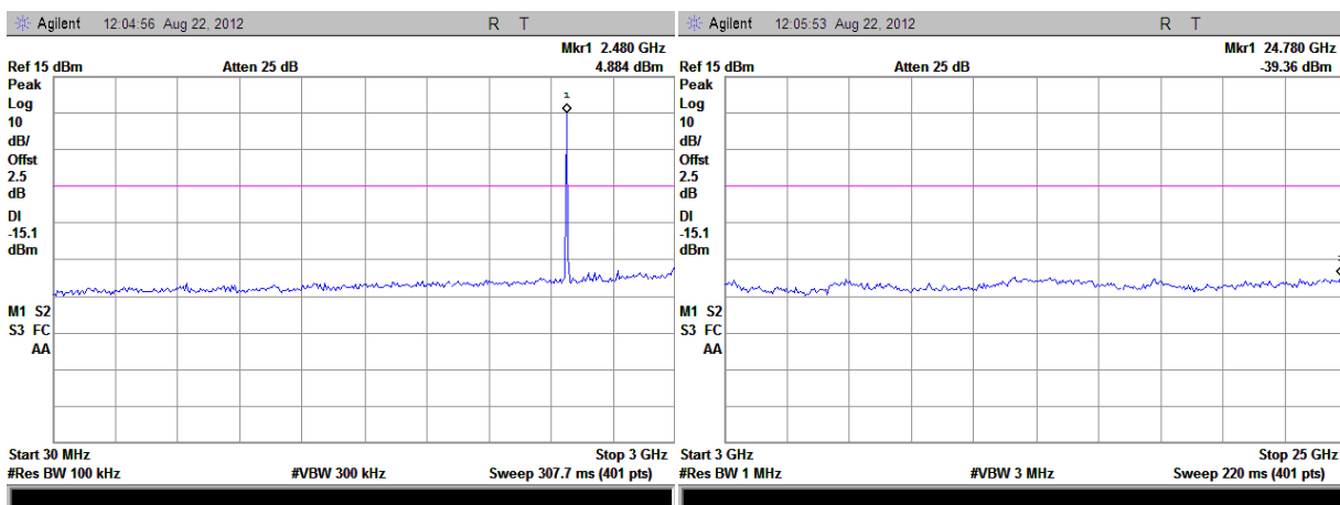
(Plot C.1: Channel = 39, 30MHz to 3GHz)
