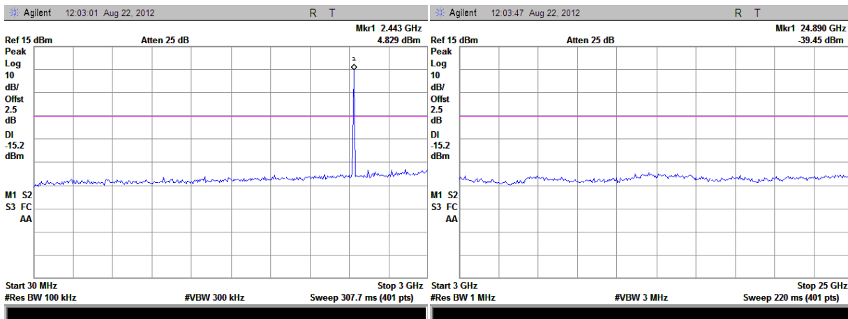
(Plot B.1: Channel = 19, 30MHz to 3GHz)
