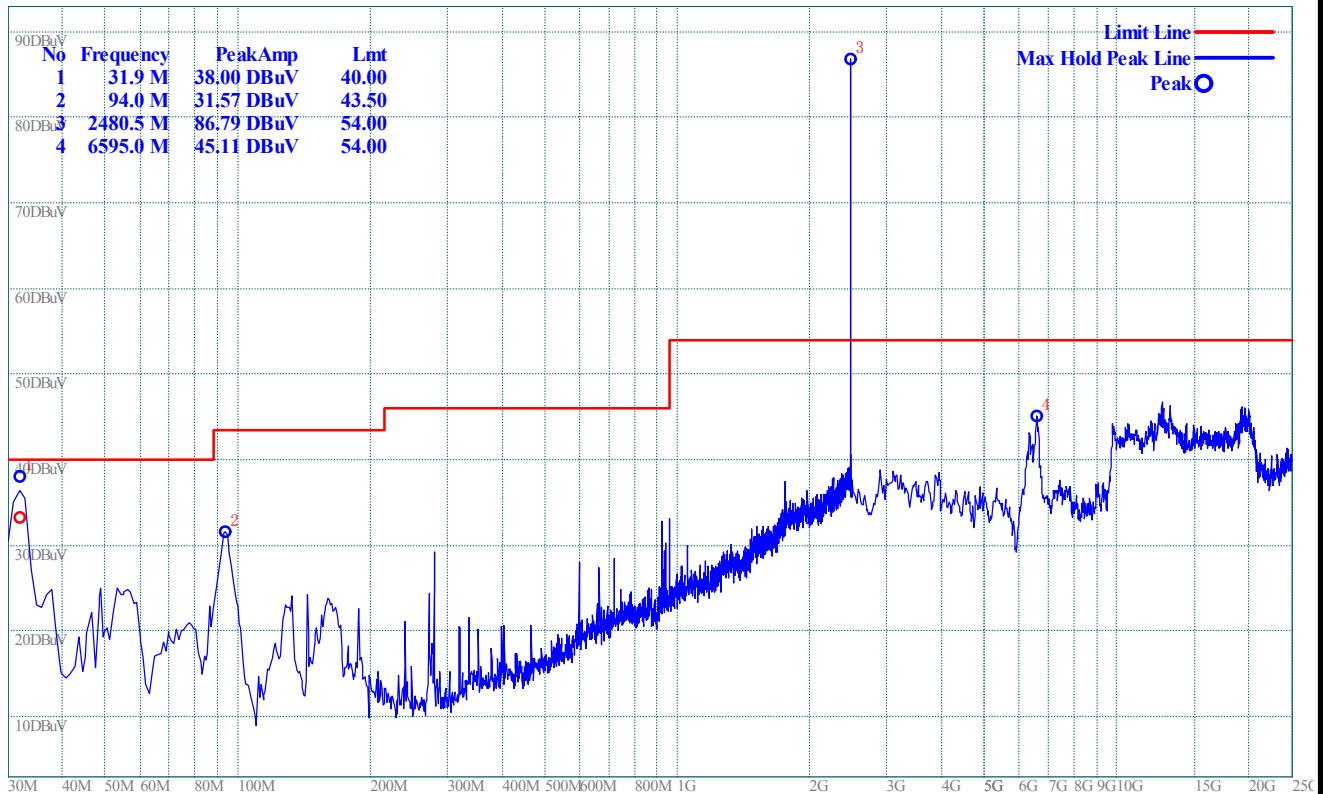
(Plot C.2: 30MHz to 25GHz, Antenna Vertical @ 11/4-DQPSK, channel 78)
