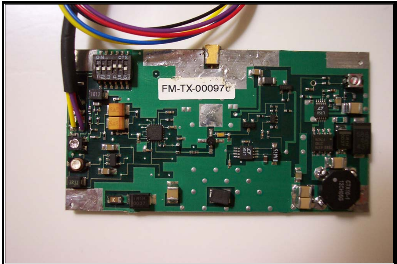
Photograph 4: PCB Top View
