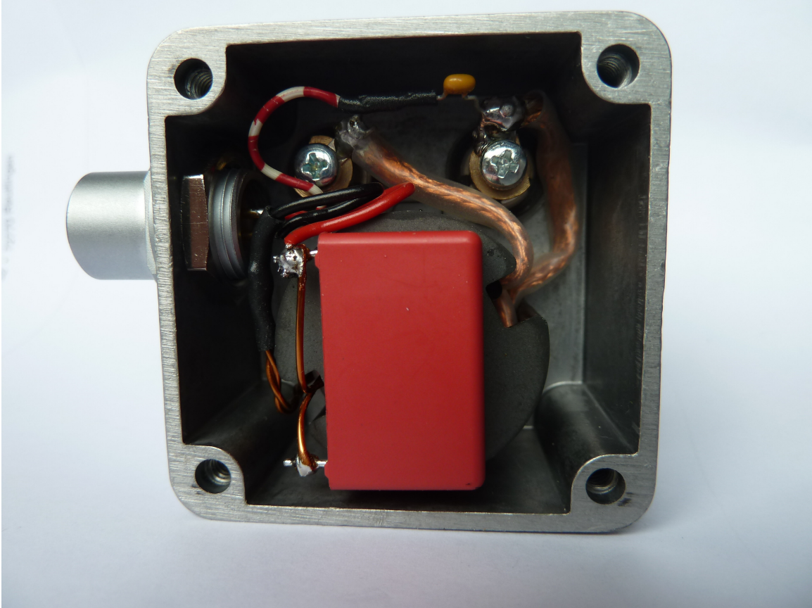
Photo 3 – Internal View of the Stator Assembly
