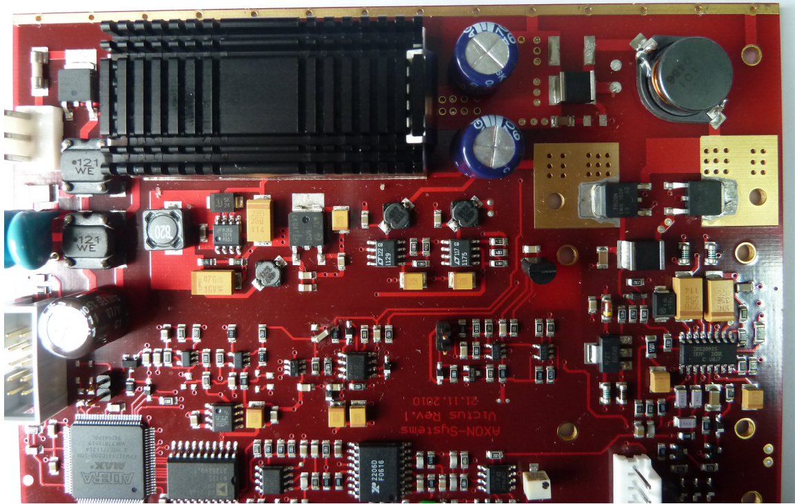
Photo 1 – J1 Controller Circuit Board Containing the 23 kHz Transmitter Top Side
