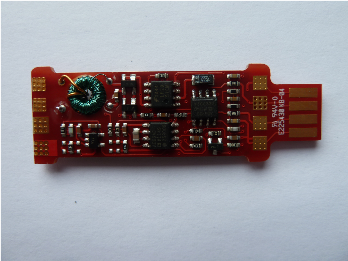
Photo 4 – Top Side Internal View of the Rotor Unit containing the 10.7 MHz Transmitter
