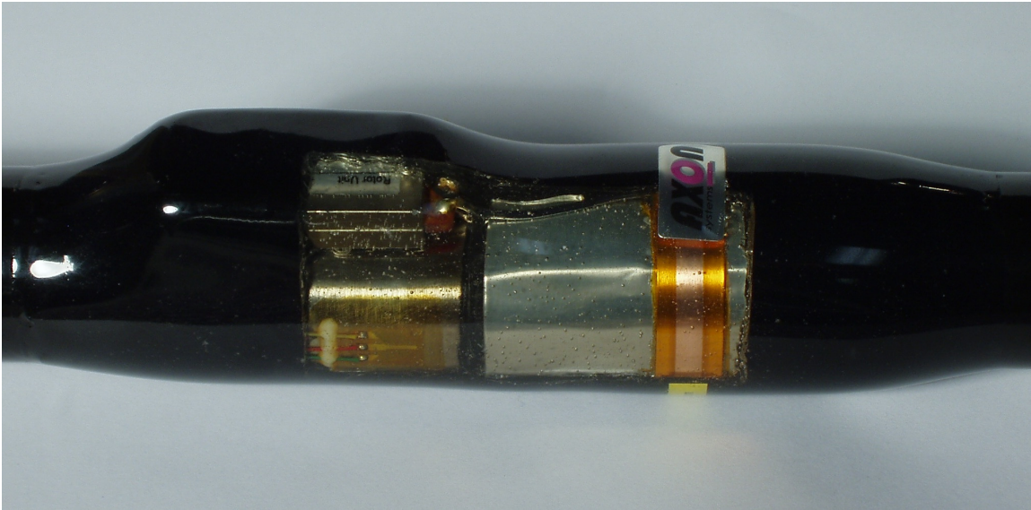
Photo 3 – Sealed Rotor Unit Mounted to Drive Shaft
