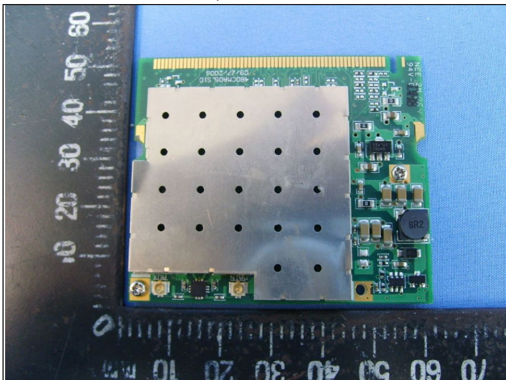
EUT Sample for U.FL connector
