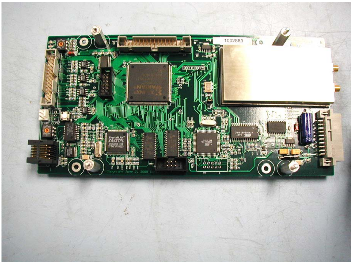
Figure 3: Radio card with Shield
