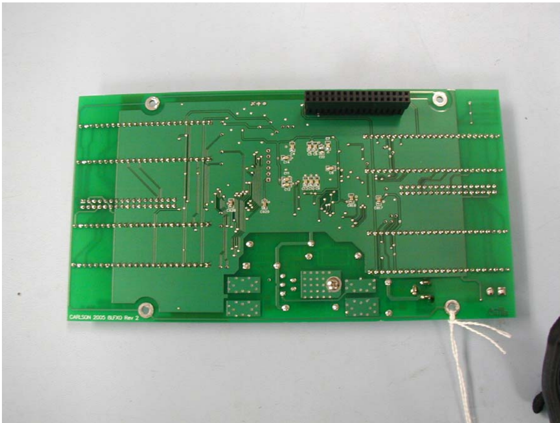
Figure 2: Bottom view of power supply and DS0 interface
