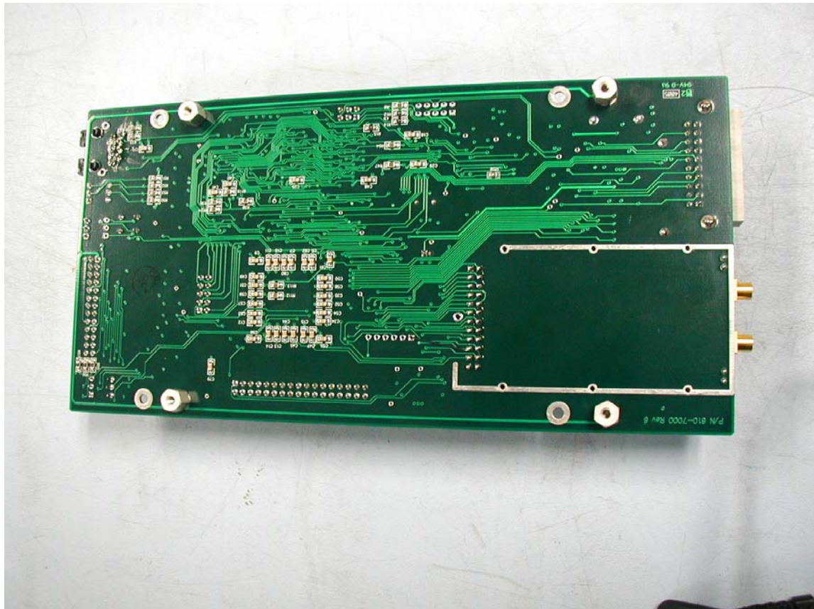
Figure 5: Radio card bottom view
