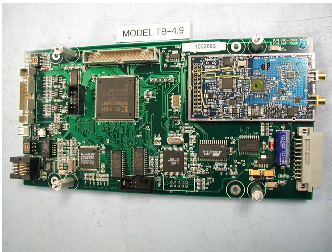
Figure 4: Radio top view no shield
