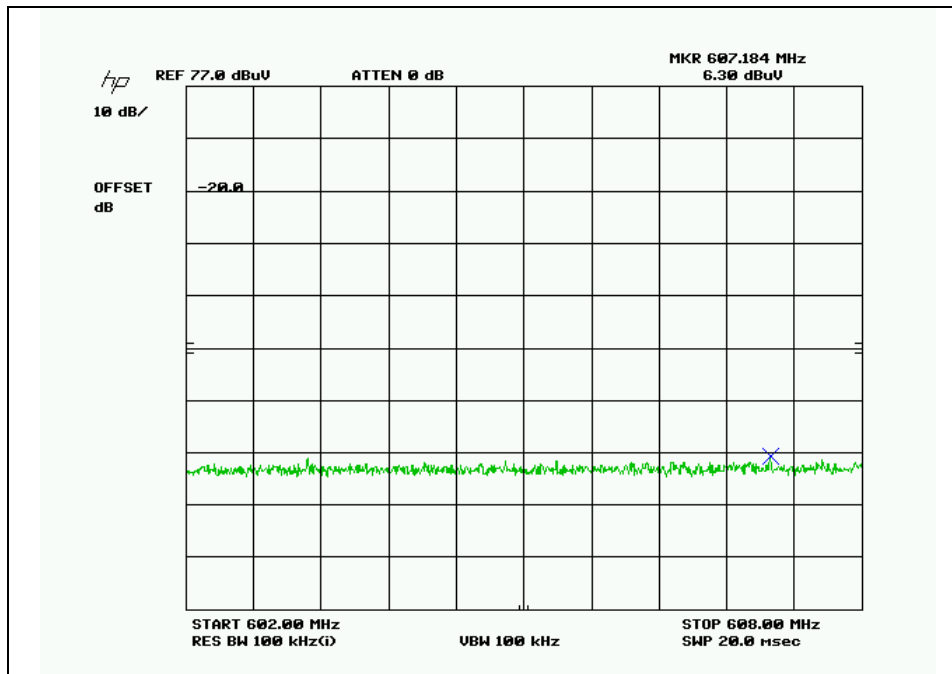
602-608 MHz, Horizontal, (with TX at CH 39), PK Det.
