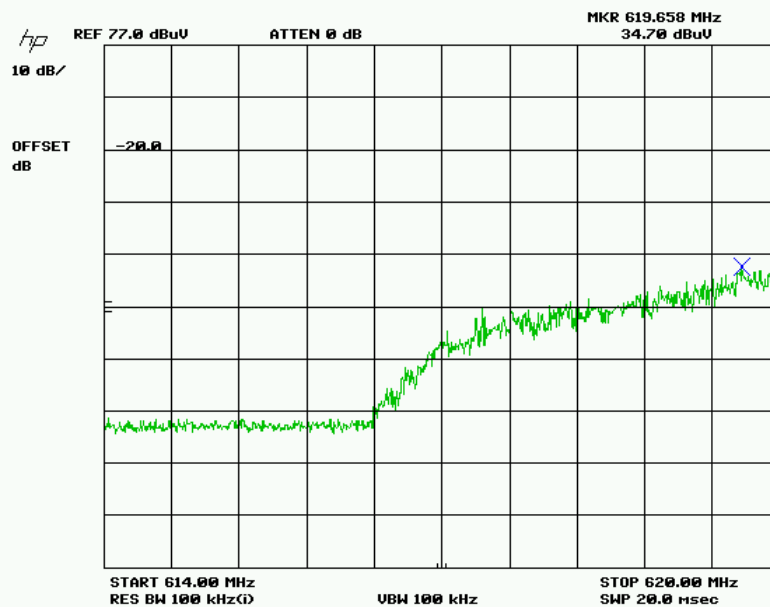
614-620 MHZ, Vertical, (with TX at CH 39), PK Det(add + 30dB for pad)
