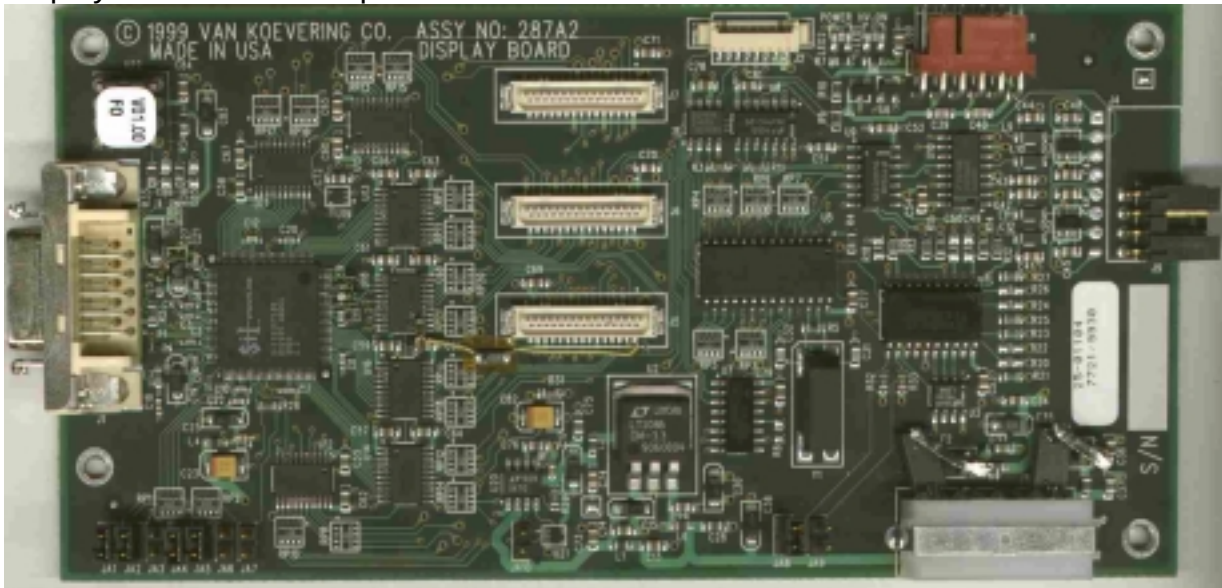
Display PC Board – Component Side
